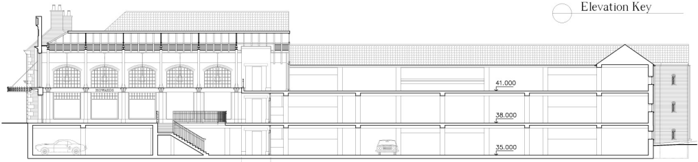
5 Section C 46
