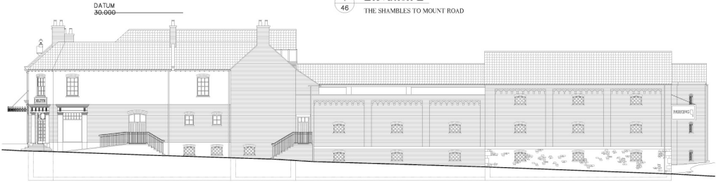
1 Elevation E 46 THE SHAMBLES TO MOUNT ROAD
